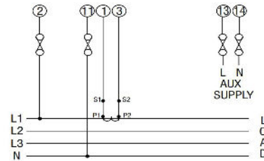
Single Phase
