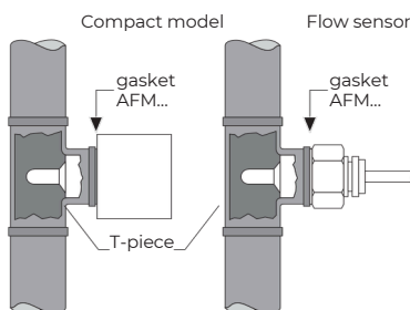
1. Installation in rising pipe
