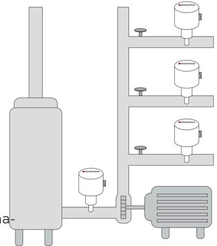
Run-dry protection of a feed pump
