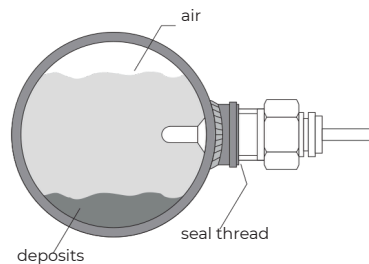
2. Lateral installation
