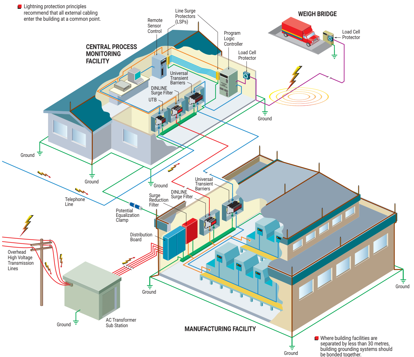
nVent ERICO Electrical Plan of Protection applied to a manufacturing facility. Surge and transient protection principles applied to an entire facility rather than individual pieces of equipment.
