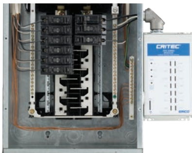
Typical Installation
